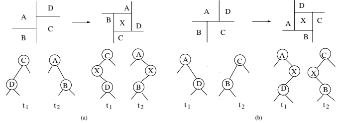
Figure 9: Mapping between mosaic floorplan and non-slicing floorplan
